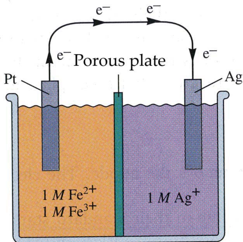
Figure 6- 4: The galvanic iron/silver cell Schematic setup of the Ag + /Ag and Fe 2+ /Fe 3+ cell.
