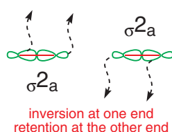
\sigma bond reacting antarafacially
